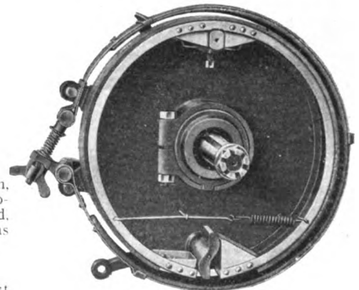
INTERNAL AND EXTERNAL BRAKES.
